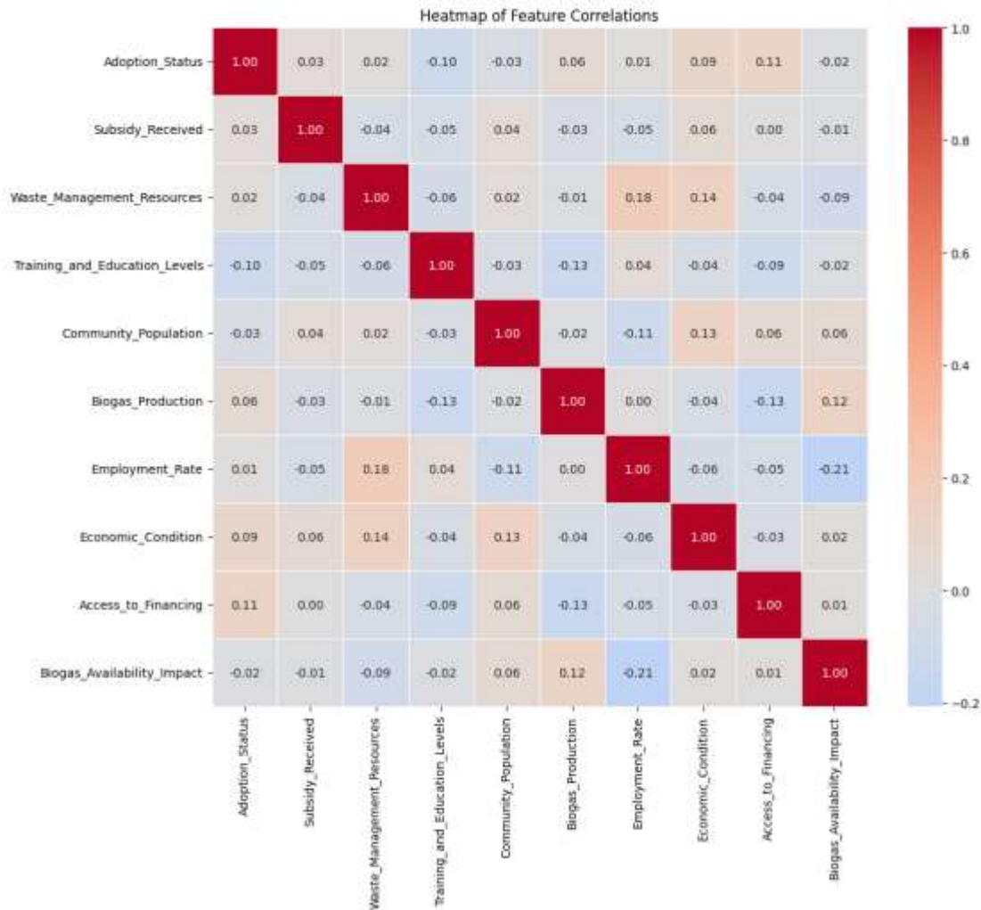
Fig. 1: Feature Correlation
