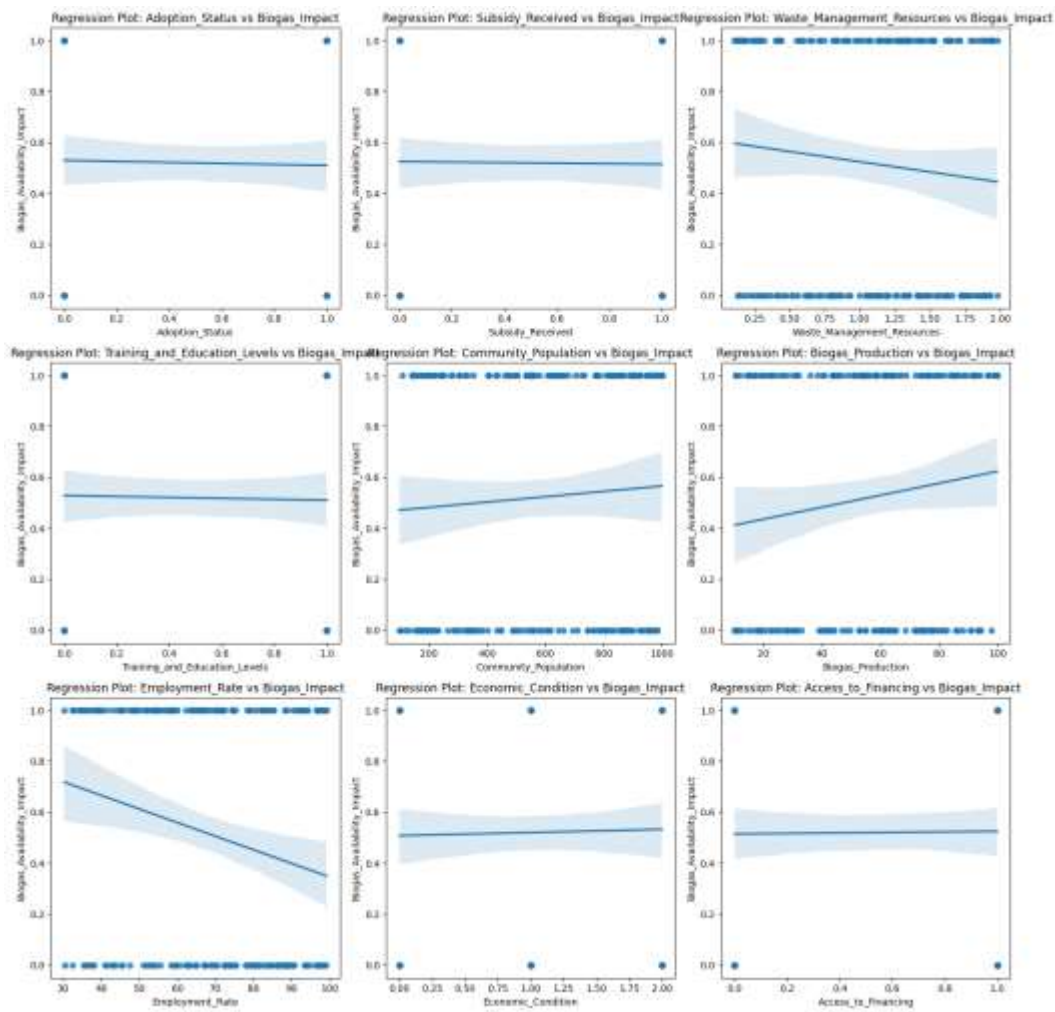
Fig.3: Regression plot of features
